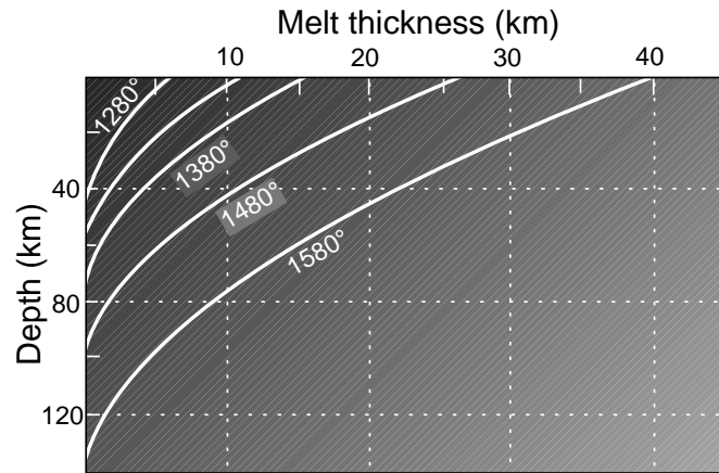
Figure 7.8: Thickness of melt (measured as a vertical column in kms) present below the given indicated depth produced by the adiabatic decompression of garnet peridotite for different potential temperatures (after McKenzie and Bickle, 1988). For the modern day mantle with a potential temperature of 1280°C melting will not occur at depths less than about 45 km. Adiabatic decompression of the modern day mantle by the complete removal of the overlying lithospheric "lid" (for example at a spreading ridge) will result in the generation of a 7 km pile of MORB-like melt (i.e., the oceanic crust).
