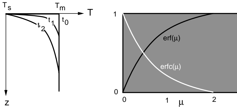
Figure 7.2: Schematic thermal structure of the ocean lithosphere treated as a problem of the cooling of a semi-infinite half space. (a) shows the thermal structure at the ridge ( t_0 ) where asthenosphere at temperature T_m is juxtaposed with ocean waters at temperature T_s . The thermal structure at successive distances away from the ridge where cooling of the initial temperature discontinuity in the semi infinite half space has led to thickening of the ocean lithosphere is shown by the curves t_1 and t_2 . (b) shows the error function ( \operatorname{erf} ) and complimentary error function ( \operatorname{erfc} = 1 - \operatorname{erf} ).
