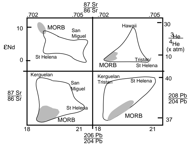
Figure 7.9: The range of radiogenic isotopic compositions (Nd, Sr, Pb and He) of oceanic basalts. The stippled area is the compositional range of Mid Ocean Ridge Basalts (MORB). The remaining envelope is the region of ocean island basalts (OIB). Clearly the OIB sources of the whole Earth are not all the same (from Allegre, 1987)
