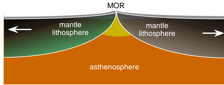
Figure 7.1: Schematic structure of the ocean lithosphere. The ocean lithosphere consists of about 6-7 km thick crust (heavy stipple), and the mantle lithosphere (intermediate stipple) which thickens with age (and hence distance away from the ridge as indicated by arrows). Light stipple show the region of decompression melting beneath the ridge. Stream lines in the asthenosphere may be largely decoupled from the motion of the overlying lithosphere (see Section 5.5), although asthenosphere must undergo decompression immediately beneath the ridge.
