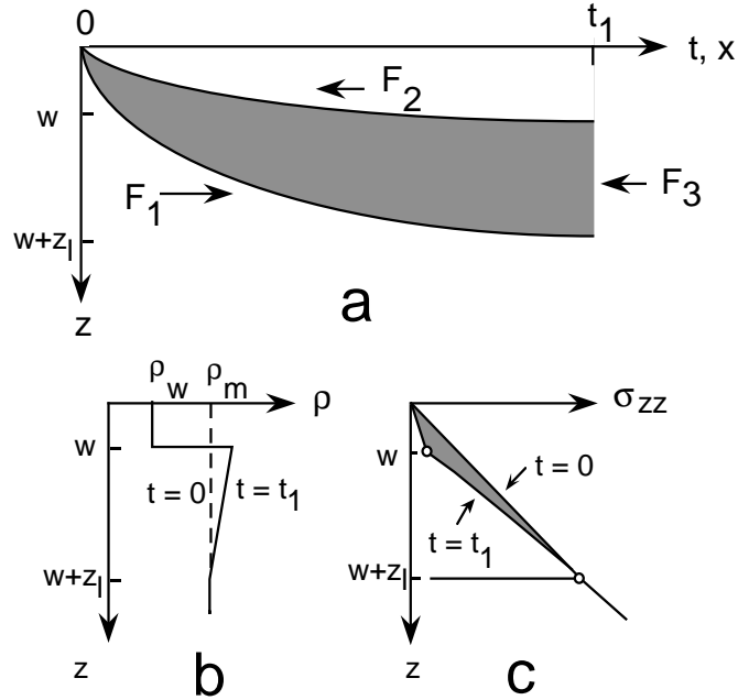
Figure 7.4: Ridge push is the force resulting from isostatically induced topographic gradients in the oceanic lithosphere. (a) shows a diagrammatic representation of the force balance between a ridge and ocean lithosphere at age t = t_1 . (b) shows the density distribution appropriate to (a). The dashed line shows the vertical density structure at t = 0 . The solid line shows the vertical density structure at t = t_1 . (c) shows the graphical solution to the force balance.
