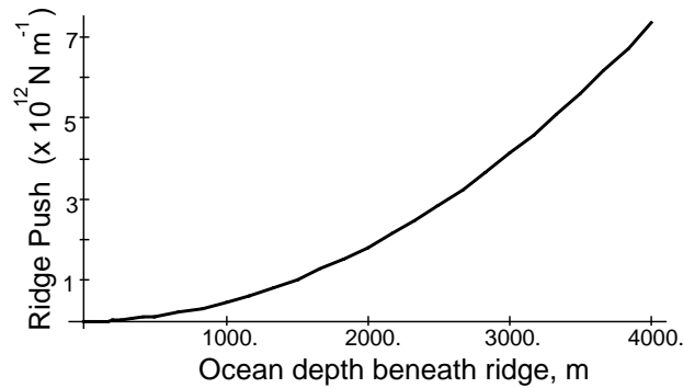
Figure 7.5: Ridge push, F_R , plotted as function of depth of ocean beneath ridge crest, w .
