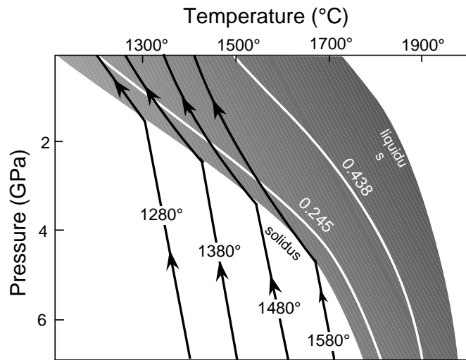
Figure 7.7: P-T diagram showing melting field of garnet peridotite and adiabatic (isentropic) decompression paths for mantle with potential temperatures of 1280^{\circ}\text{C} , 1380^{\circ}\text{C} , 1480^{\circ}\text{C} and 1580^{\circ}\text{C} , respectively (after McKenzie and Bickle, 1988).
