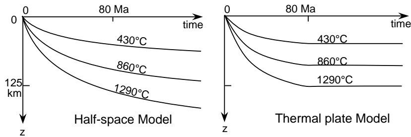
Figure 7.3: Thermal structure of the ocean lithosphere predicted by the semi-infinite half space model (a) and by the thermal plate model (b).
