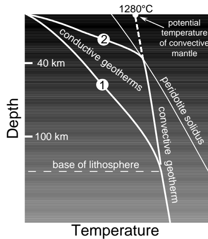
Figure 7.6: The oceanic lithosphere is characterised by its conductive geothermal gradient. The thermal gradient of the asthenosphere which is relatively well mixed (probably due to convection) is largely the isentropic temperature (adiabatic) gradient of the mantle due to volume and heat capacity ( C_p ) changes with changes in pressure (depth). The temperature at which this adiabatic temperature gradient extrapolates to the earth's surface is referred to as the potential temperature. Note that with the lithosphere of normal thickness (125 km), the solidus of the mantle peridotite nowhere intersects the geotherm but that on rifting of the lithosphere, the decompressed asthenosphere's adiabat intersects the solidus at about 40 km depth.
